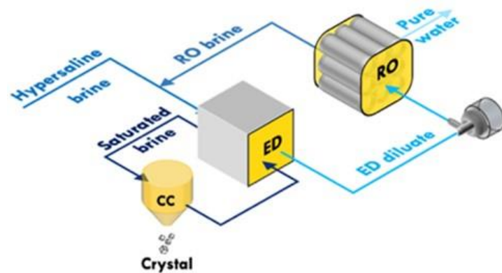
Figure S2. Basic diagram of Electrodialysis system.
