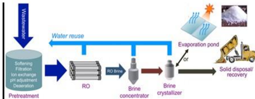
Figure S1. Diagram of modern methods of saline brine reclamation.
