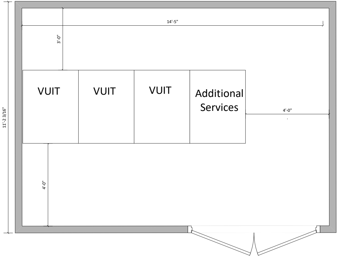
Typical Core Distribution Room Layout
