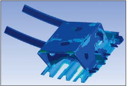
Existing Fan Support Bracket Stress Analysis.
