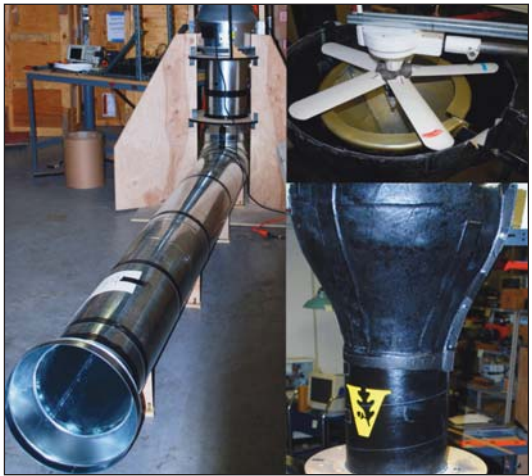
(Clockwise from left) Intake duct and inline fan; Wind turbine with ogive; Redesigned exhaust stack funnel.
