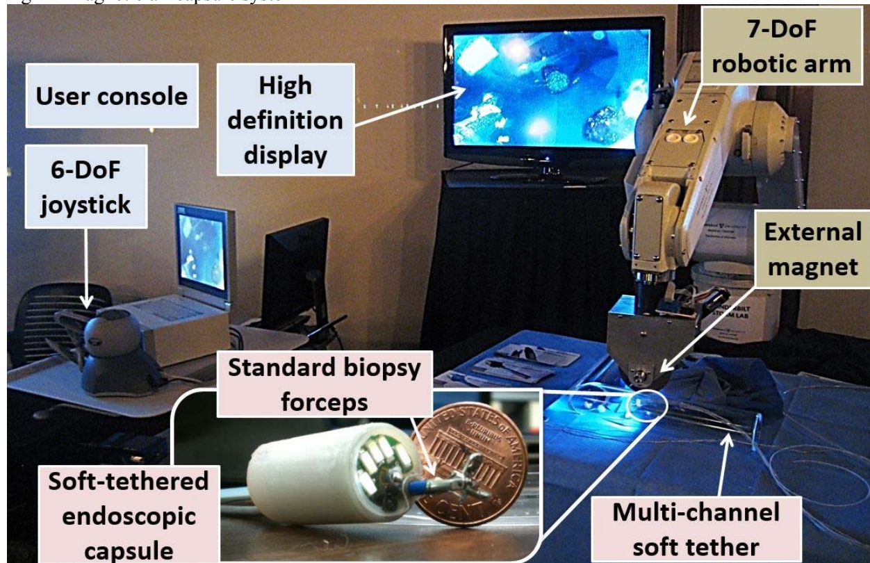
Fig 1 – Magnetic air capsule system
