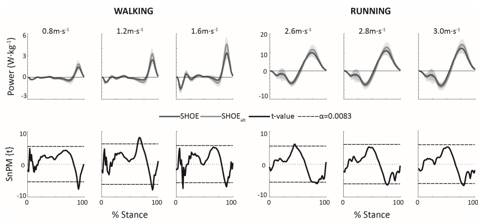
Figure 2. SHOE vs. SHOE alt : ankle joint complex power estimates for walking and running using two shoe-applied calcaneal tracking marker set configurations: SHOE (dark grey) and SHOE alt (light grey). Data are presented as mean±s.d. (shaded regions), for stance phase. Statistical non-parametric (SnPM) mapping t-values (black solid line) are displayed in lower plots, with an adjusted alpha level threshold (black dashed line).
