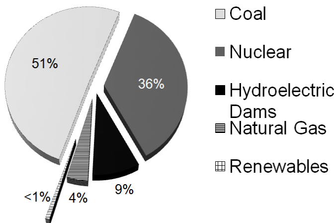
Figure 3.1. TVA's Fuel Mix, Calendar Year 2010 14 .
