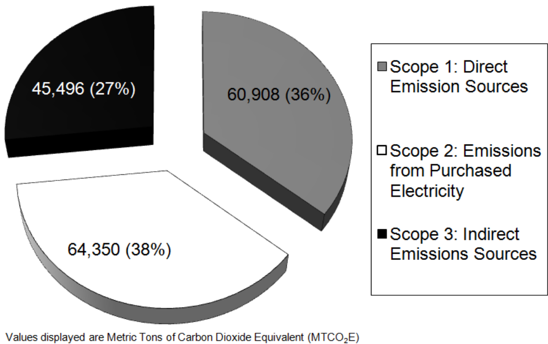
Figure 5.3. GHG Emissions Sources by Scope from Patient Care Areas, Calendar Year 2010.
