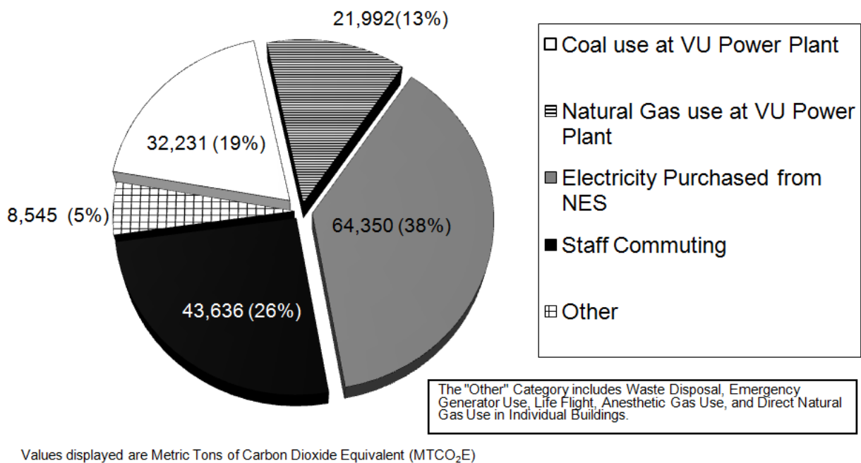
Figure 5.2. GHG Emissions Sources from Patient Care Areas, Calendar Year 2010.
