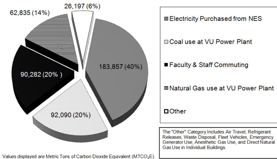
Figure 6.2. GHG Emissions Sources, Calendar Year 2010.
