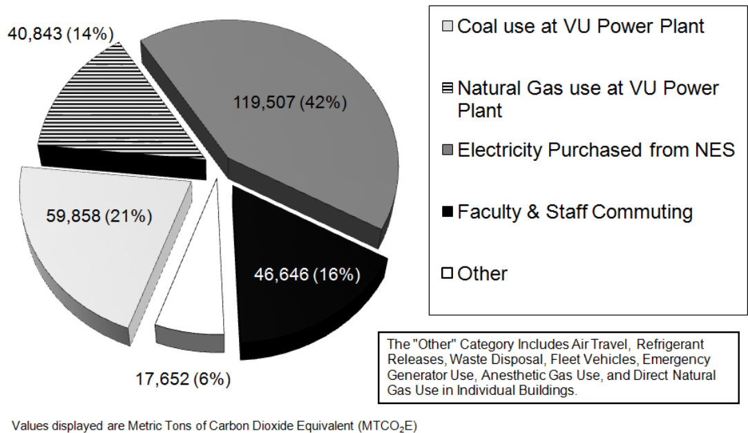
Figure 4.2. GHG Emissions Sources from Academic and Research Areas, Calendar Year 2010.
