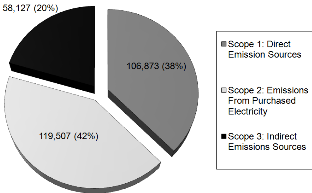
Figure B.3. Vanderbilt Academic and Research Area GHG Emissions Sources by Scope, Calendar Year 2010.
