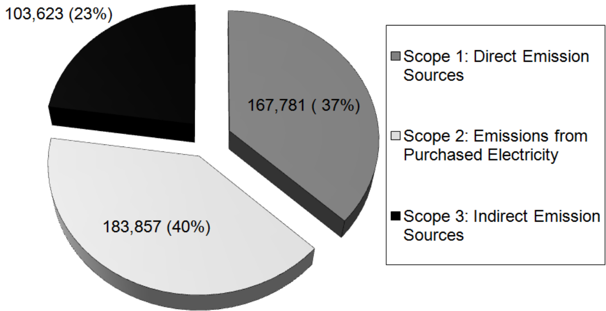
Figure B.2. Vanderbilt GHG Emissions Sources by Scope, Calendar Year 2010.
