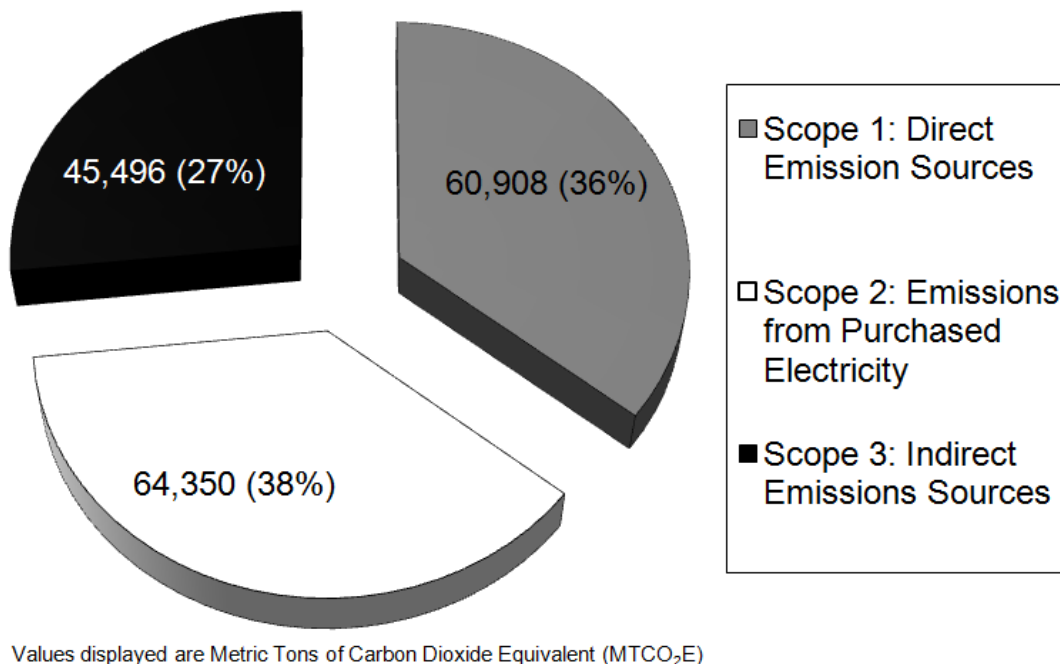
Figure B.4. Vanderbilt Patient Care Area GHG Emissions Sources by Scope, Calendar Year 2010.
