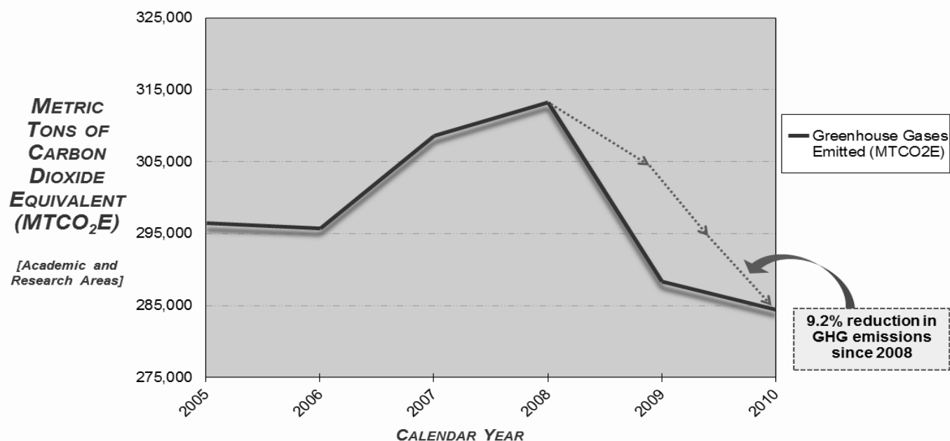
Figure 4.1. GHG Emissions from Academic and Research Areas, Calendar Years 2005-2010.
