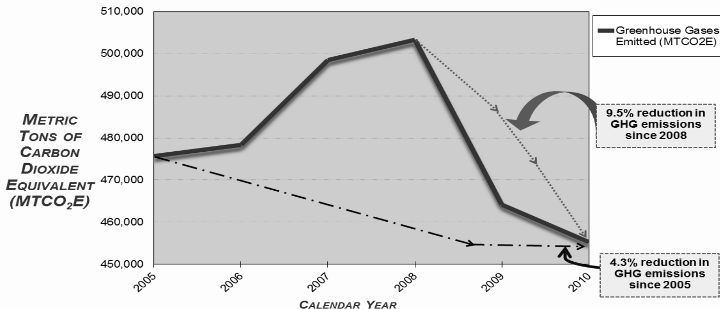
Figure 6.1. Total Vanderbilt GHG Emissions, Calendar Years 2005-2010.
