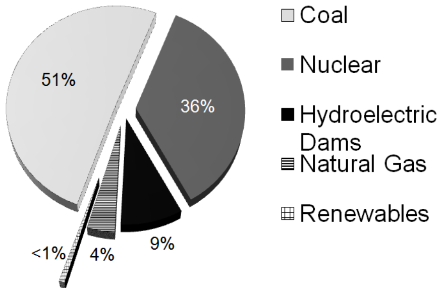
Figure B.5. TVA Fuel Mix, Calendar Year 2010.
