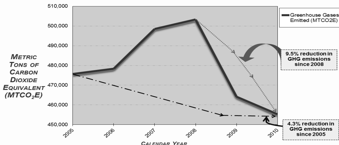
Figure ES.1. Total Vanderbilt GHG Emissions, Calendar Years 2005-2010.
