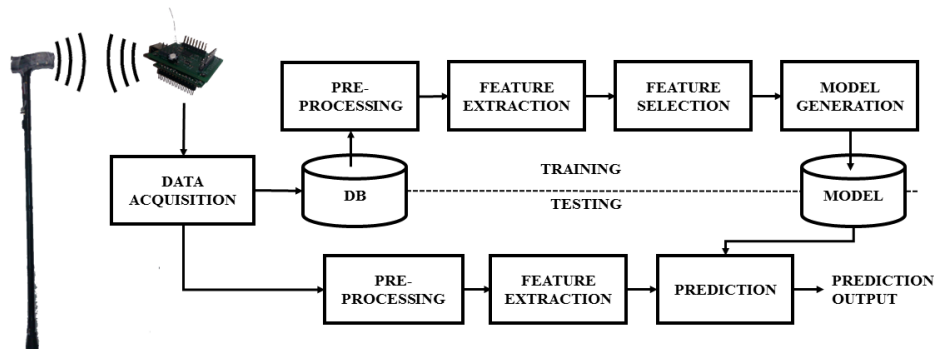
Figure 4. The overall system architecture.
