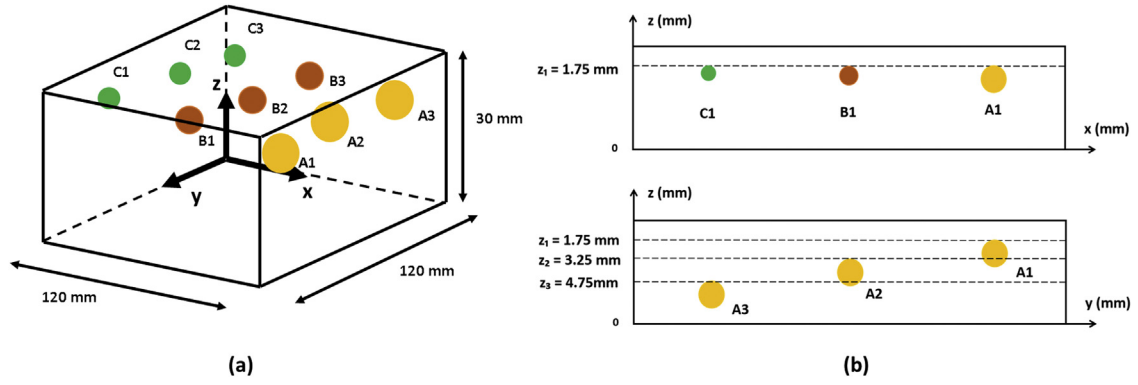
Fig. 8. Dimensions of the fabricated phantoms with the embedded lump locations (a) and their relative depth (b).
