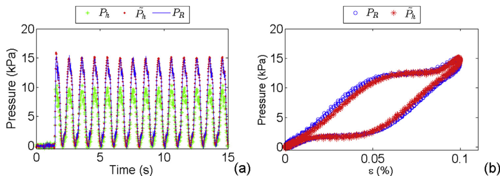
Fig. 6. The Wireless Palpation Probe (WPP) head is tested under a dynamic strain at a frequency of 1 Hz (a) and the results of the stress–strain curve for the loading unloading cycles (b).
