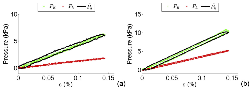
Fig. 7. Palpation of the two different stiffness samples. Unfiltered sensor data (in red) and filtered sensor data (in black). (For interpretation of the references to color in this figure legend, the reader is referred to the web version of the article.)
