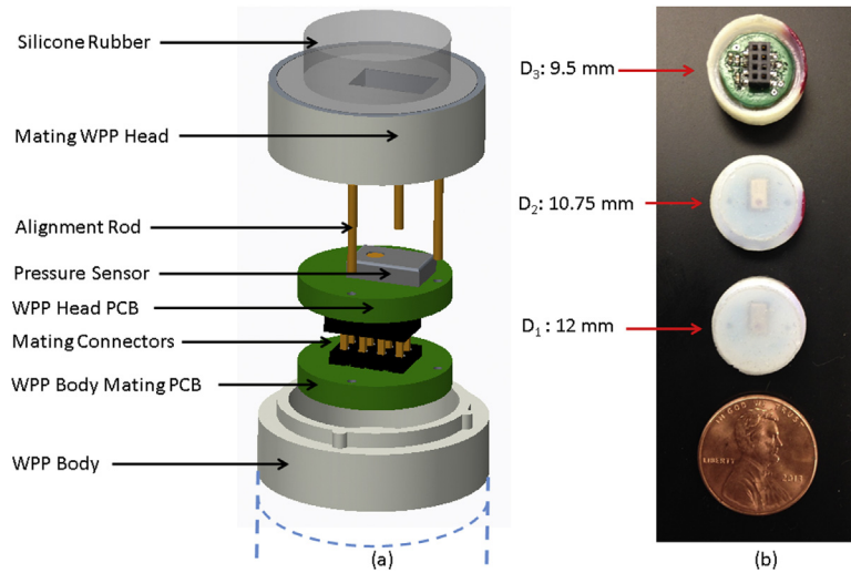
Fig. 1. The WPP head exploded view (a), the fabricated heads of different diameters (b).
