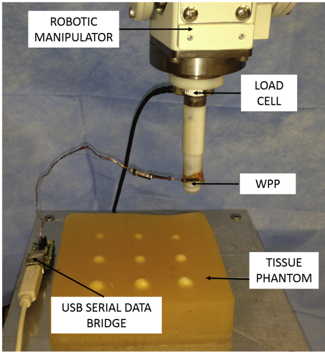
Fig. 4. The platform to assess the WPP head calibration.
