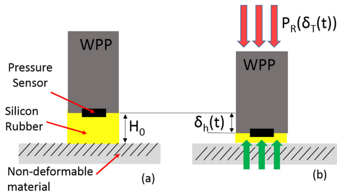
Fig. 2. Schematic diagram of the calibration procedure at contact (a) and at an arbitrary instant of time (b) for a non-deformable material.
