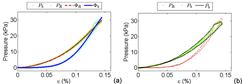
Fig. 5. The raw pressure data, the reference pressure, and their numerical functions' interpolations (a), the raw and calibrated pressure data compared with the reference pressure P_R (b).
