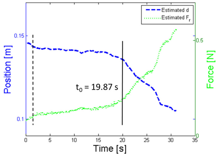
Figure 10. Plot of the modules of F_r and d acquired during the in vivo trial. The dashed vertical line indicates the instant when the EPM was moved closer to the capsule, while the solid vertical line indicates the instant when capsule motion started.
