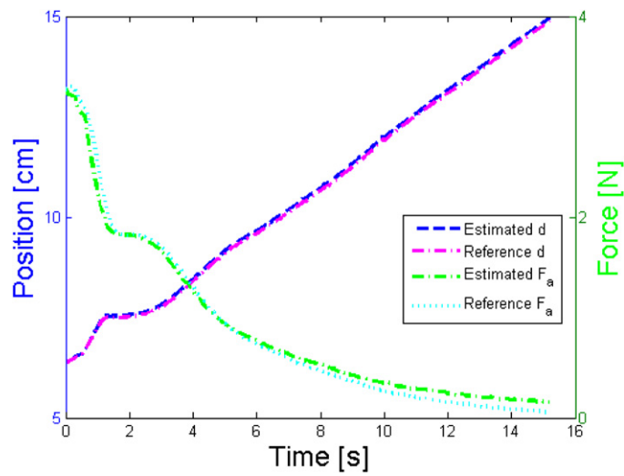
Figure 6. Modules of the estimated force F_a , the reference force along z_c , the estimated position d , and the reference position as measured by the robotic manipulator encoders for part of a trial where the EPM was moved mainly along the z_c -axis (i.e., from \{x_c = 8 \text{ mm}, y_c = -10 \text{ mm}, z_c = 62 \text{ mm}\} to \{x_c = 8 \text{ mm}, y_c = -5 \text{ mm}, z_c = 148 \text{ mm}\} ).
