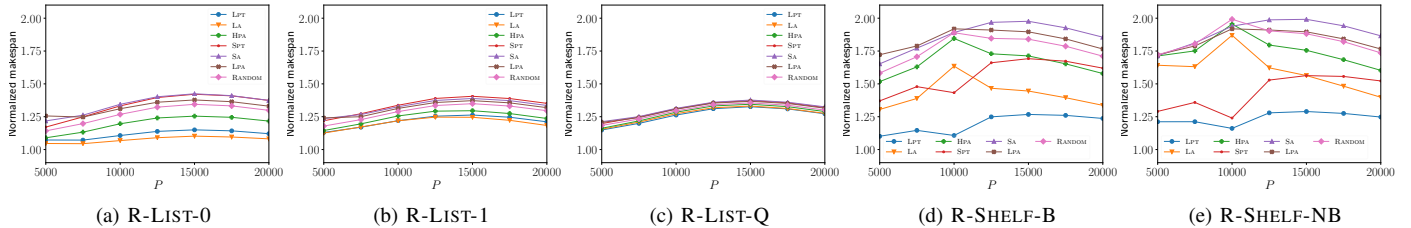
Fig. 3. Normalized makespans of different heuristics and priority rules over 30 sets of jobs when P varies between 5000 and 20000, and \bar{q} = 0.3 .
