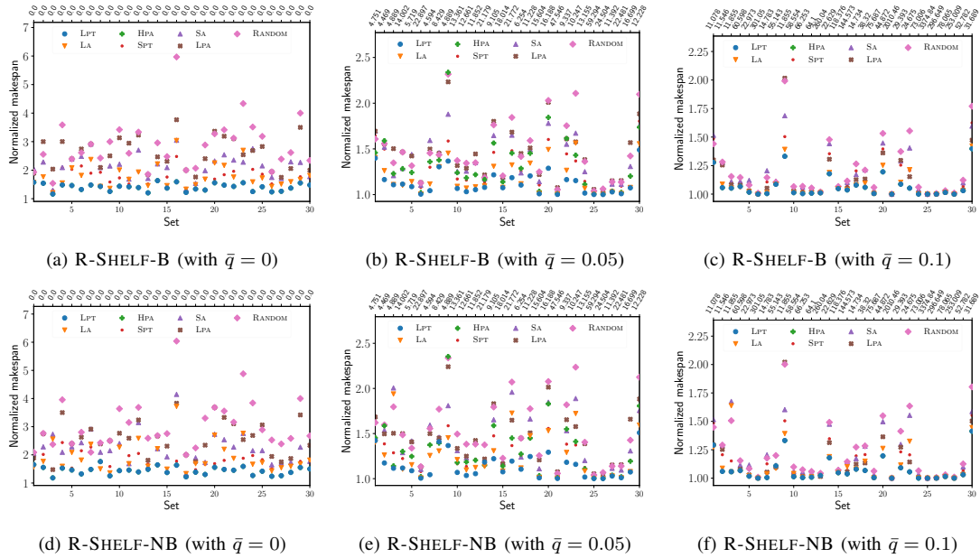
Fig. 6. Performance of shelf-based heuristics for 30 job sets using the Mira trace logs (June 2019) with and without failures. Each row represents a different heuristic (R-SHELF-B and R-SHELF-NB), and each column represents a different failure probability ( \bar{q} = 0 , \bar{q} = 0.05 and \bar{q} = 0.1 ). The average number of failures for each job set is indicated on top of each plot.
