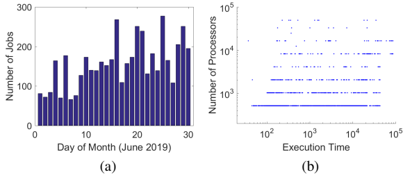
Fig. 1. Data from the trace logs of the Mira supercomputer.
