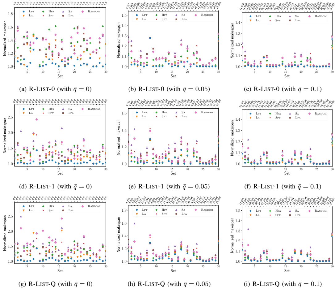
Fig. 5. Performance of list-based heuristics for 30 job sets using the Mira trace logs (June 2019) with and without failures. Each row represents a different heuristic (R-LIST-0, R-LIST-1 and R-LIST-Q), and each column represents a different failure probability ( \bar{q} = 0 , \bar{q} = 0.05 and \bar{q} = 0.1 ). The average number of failures for each job set is indicated on top of each plot.
