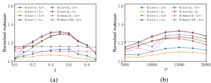
Fig. 4. Comparison of different heuristics with the best priority rules LPT and/or LA when: (a) \bar{q} varies between 0 and 0.9, and P = 10000 ; and (b) P varies between 5000 and 20000, and \bar{q} = 0.3 .
