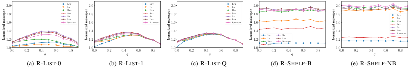
Fig. 2. Normalized makespans of different heuristics and priority rules over 30 sets of jobs when \bar{q} varies between 0 and 0.9, and P = 10000 .
